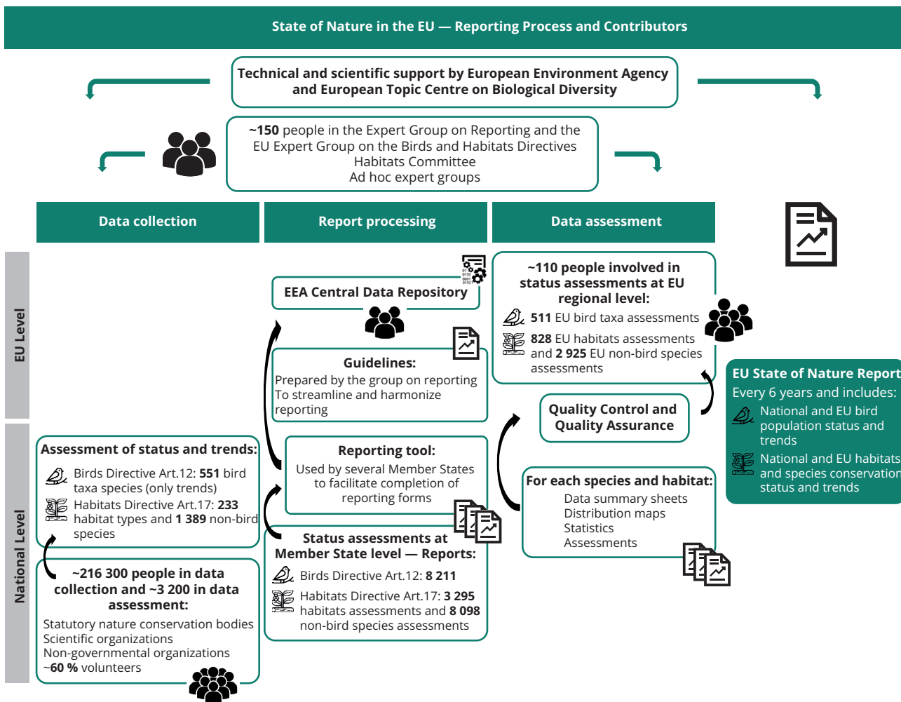
Figure 1.1 The nature directives' reporting process
