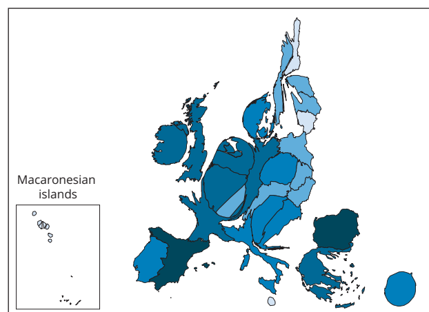
Map 2.2 Number of reported wintering taxa per country
