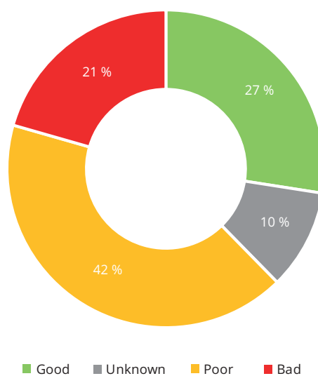
Figure 3.9 Conservation status of species at EU level
